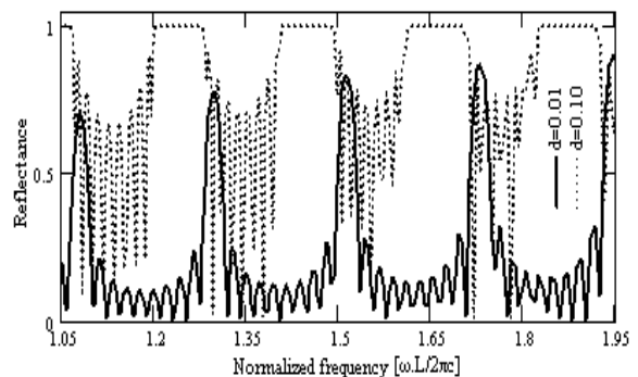
Figure 5: Reflection Spectra: Variation of Reflectance Versus Normalized Frequency for PPC2.
