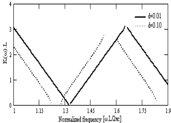
Figure 3: Dispersion relation for PPC2: Variation of Normalized Wave Vector [K(\omega).L] Versus Normalized Frequency
